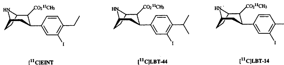
FIG. 1. Chemical structures of [ ^{11}\text{C} ]EINT, [ ^{11}\text{C} ]LBT-44 and [ ^{11}\text{C} ]LBT-14.
