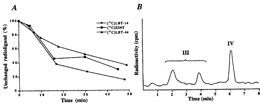
FIG. 5. Determination of unchanged radioligand in monkey plasma (% of total radioactivity versus time) of [ ^{11}\text{C} ]LBT-14, [ ^{11}\text{C} ]EINT and [ ^{11}\text{C} ]LBT-44 (A). Gradient HPLC chromatogram of a plasma sample from a Cynomolgus monkey after i.v. injection of [ ^{11}\text{C} ]EINT, obtained 16 min after administration of the radioligand. III , polar labelled metabolites; IV , [ ^{11}\text{C} ]EINT (B).
