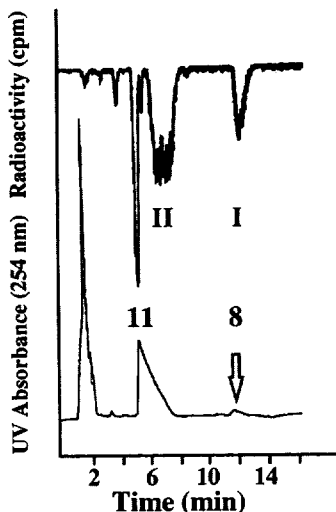
FIG. 2. Semipreparative HPLC chromatogram (U.V. and radioactivity versus time) using a Waters \mu -Bondapak-C18 column for the preparation of [ ^{11}\text{C} ]LBT-14. I , [ ^{11}\text{C} ]LBT-14; 8 , LBT-14; 11 , LBT-14 acid precursor; II , [ N\text{-CH}_3\text{-}^{11}\text{C} ]LBT-14 acid.
