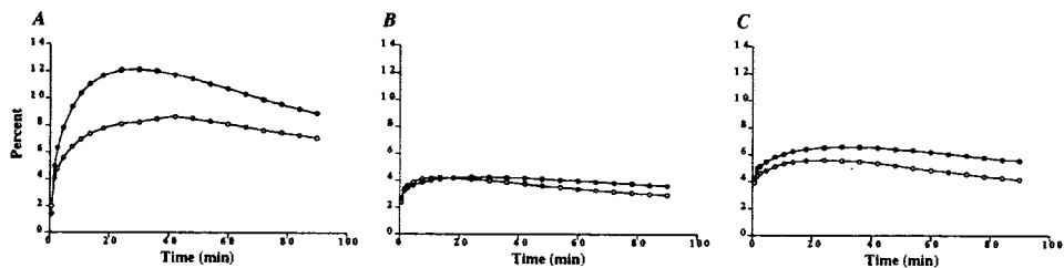
FIG. 3. Brain radioactivity in percent of injected dose of [ ^{11}\text{C} ]LBT-14 (A), [ ^{11}\text{C} ]EINT (B) and [ ^{11}\text{C} ]LBT-44 (C) in Cynomolgus monkey brain, at baseline conditions (O) and after pre-treatment with citalopram (5 mg/kg) (●).
