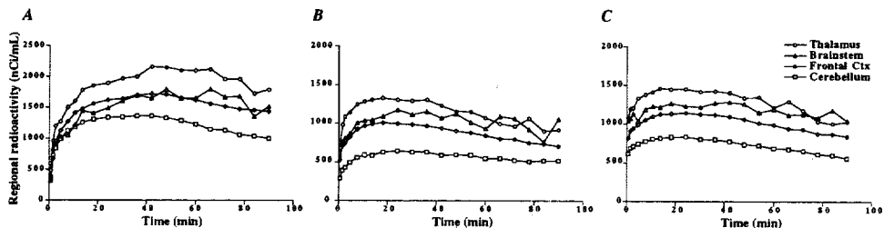
FIG. 4. Time courses for regional radioactivity (nCi/mL) in the brain of a Cynomolgus monkey after intravenous injection of [ ^{11}\text{C} ]LBT-14 (A), [ ^{11}\text{C} ]EINT (B) and [ ^{11}\text{C} ]LBT-44 (C).
